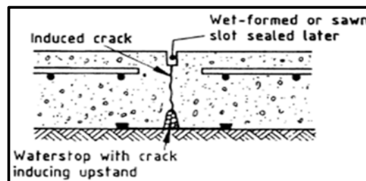
Figure 6-12: Complete Included Contraction Joints in Floors
