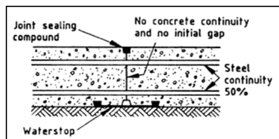
Figure 6-14: Partial Formed Contraction Joints in Floors
