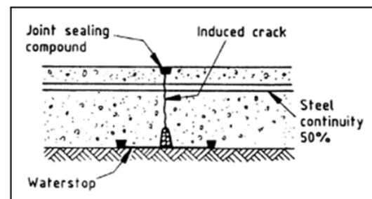
Figure 6-16: Partial Included Contraction Joints in Floors
